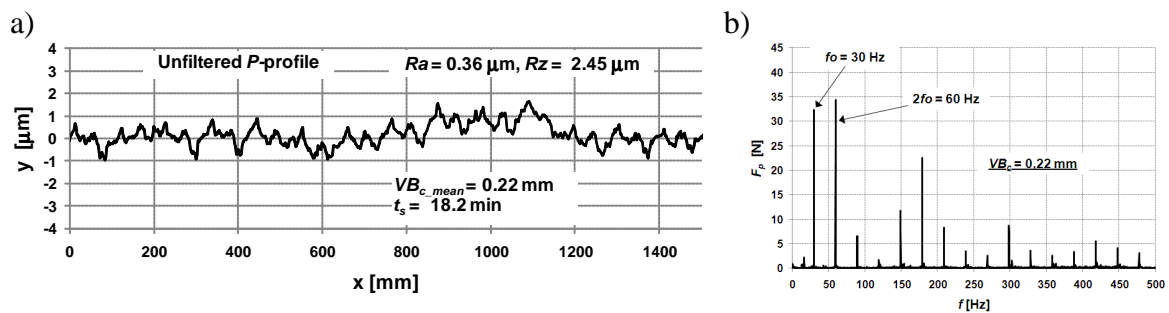
Fig. 9. a) Unfiltered P -profile; b) F_p frequency spectrum for v_c = 68 \text{ m/min} and VB_c = 0.22 \text{ mm}
